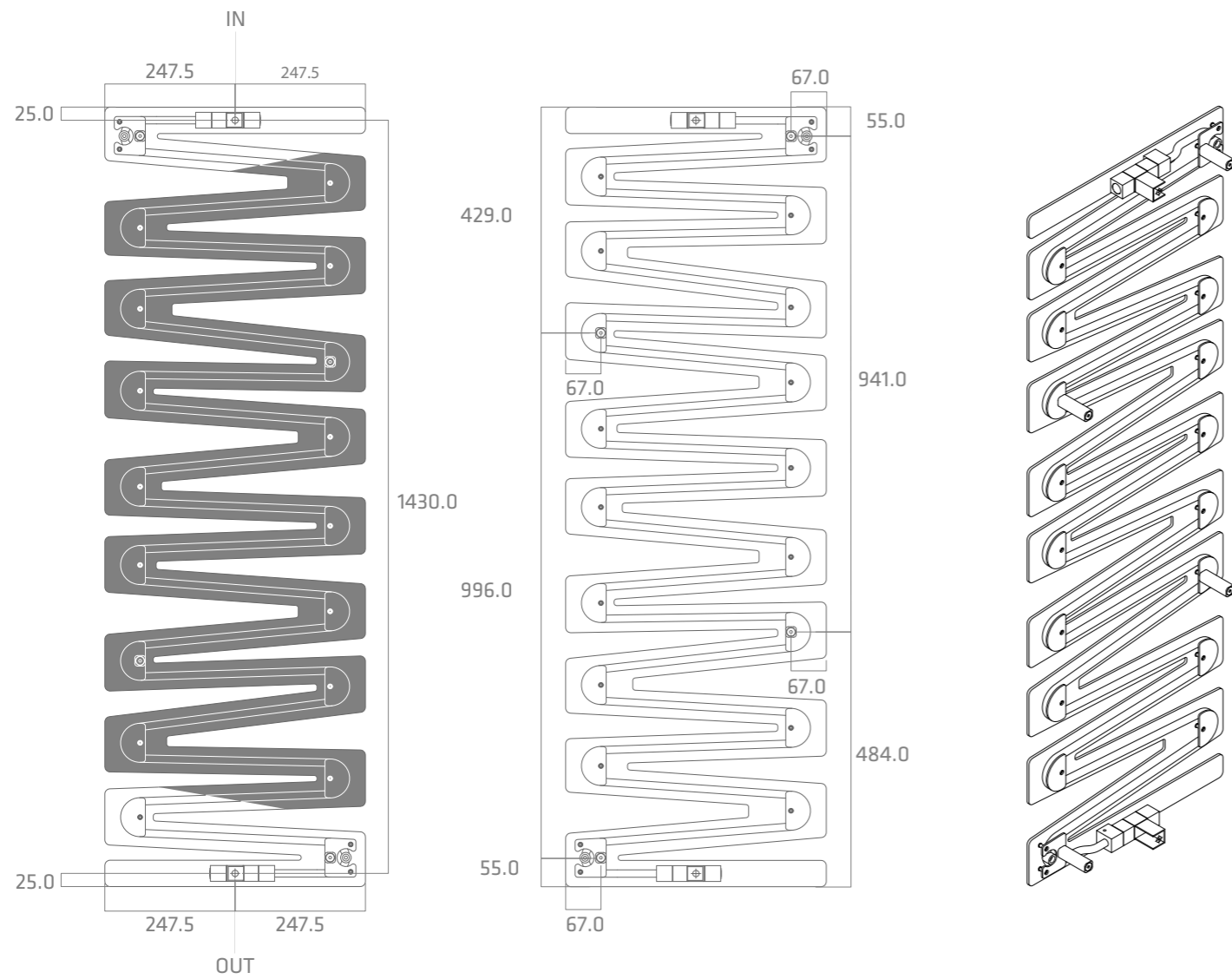
VISTA FRONTALE / FRONT VIEW quote per allaccio idraulico hydraulic connection measures
